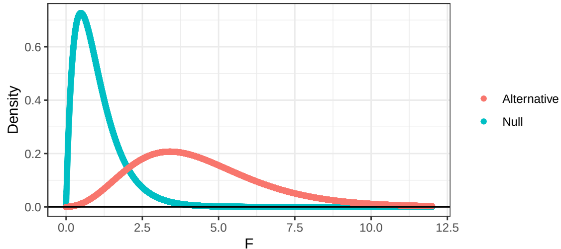
Null vs. Alternative F Distribution
